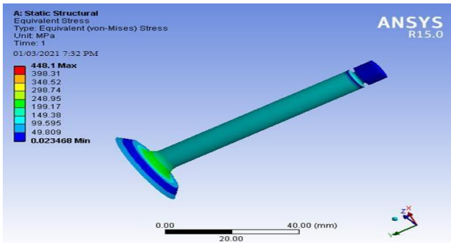
Figure10:StressofvalveusingAl+Sic(20%)
