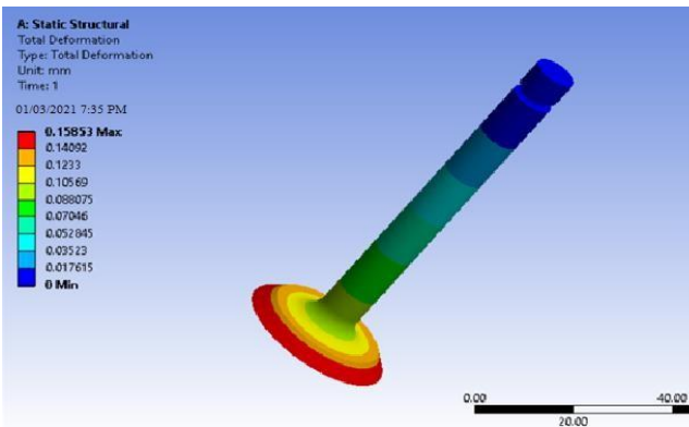
Figure11:TotalDeformationofvalveusingAl+Sic(30%)
