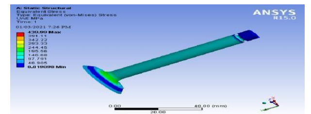
Figure 7: Stress of valve using Al+Sic(10%)
