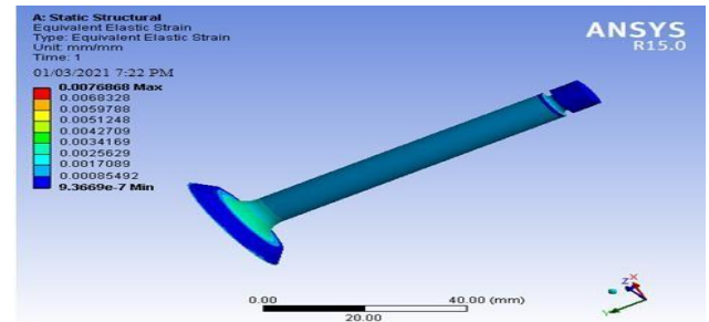
Figure 6: Strain of valve using Al+Sic(10%)
