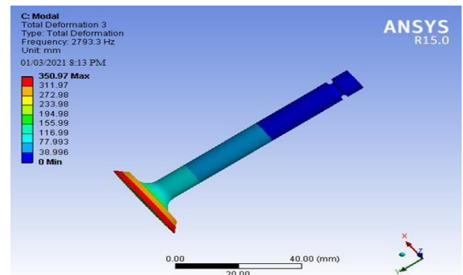
Figure16:Totaldeformationatmode3usingAISI4340
