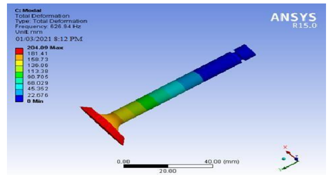
Figure14:Totaldeformationatmode1usingAISI4340
