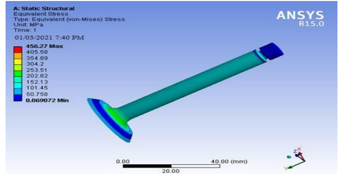
Figure13:StressofvalveusingAl+Sic(30%)
